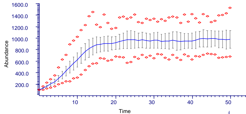
Trajectory summary
